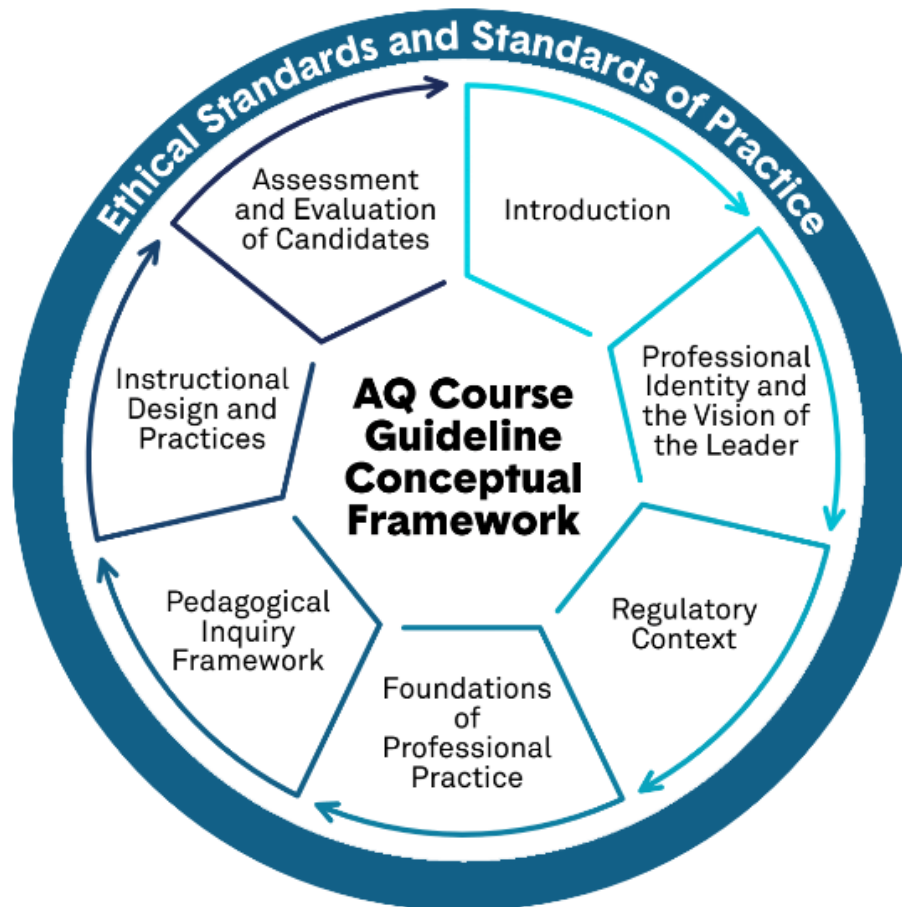
Figure 2: Conceptual Framework
