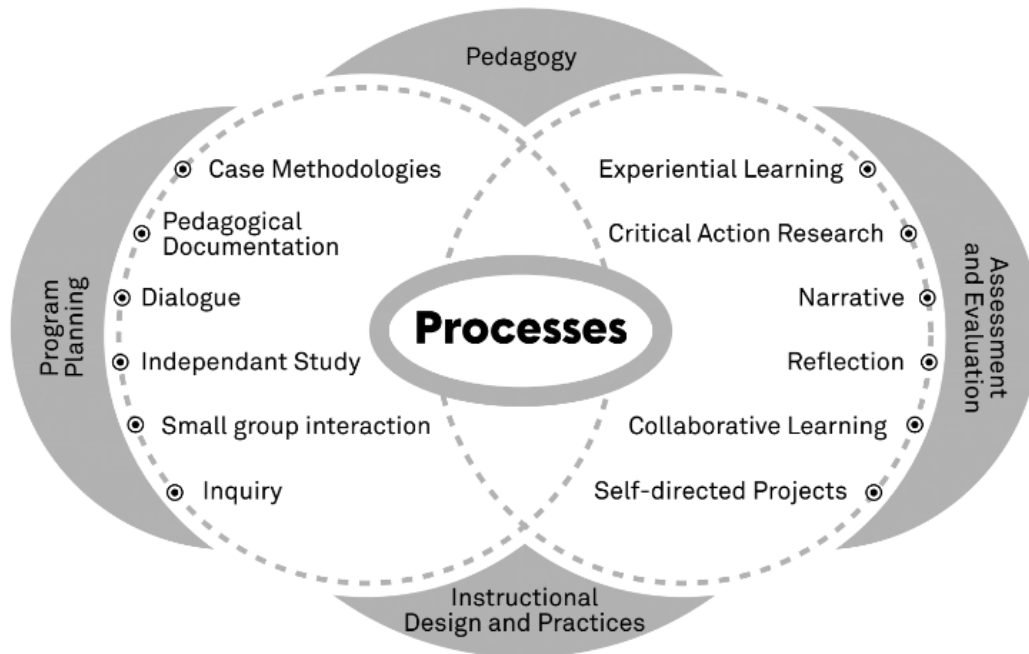
Figure 6: Instructional Processes
