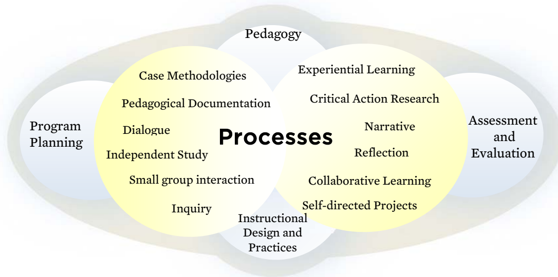
Figure 5: Instructional Processes
