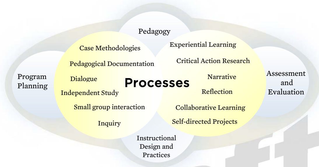
Figure 5: Instructional Processes
