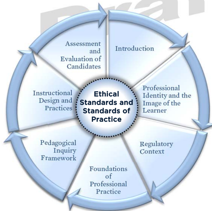
Figure 1: Conceptual Framework
